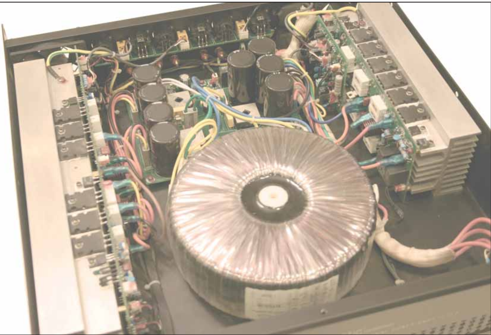
PA-1800 with rack mounting brackets
